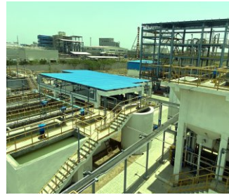
ZLD based Effluent Treatment Plant on ASP and MBBR technology
